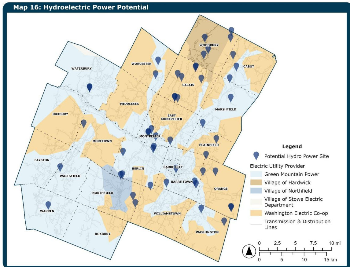
Map 16: Hydroelectric Power Potential
